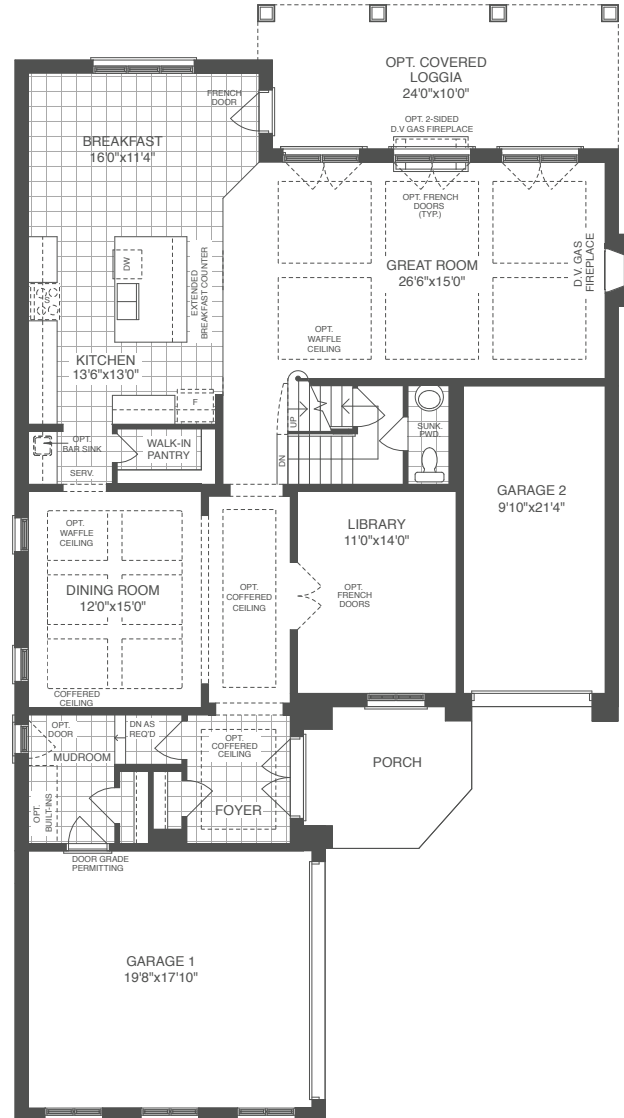
MAIN FLOOR PLAN, EL. 'A'
