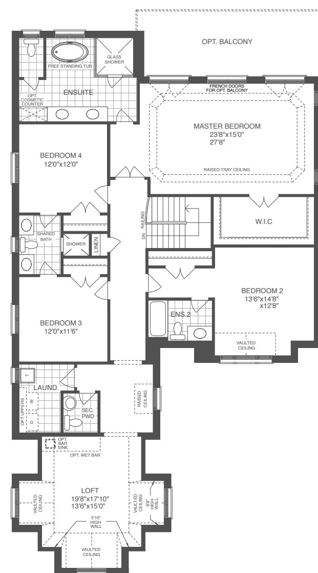
UPPER FLOOR PLAN, EL. 'A'
