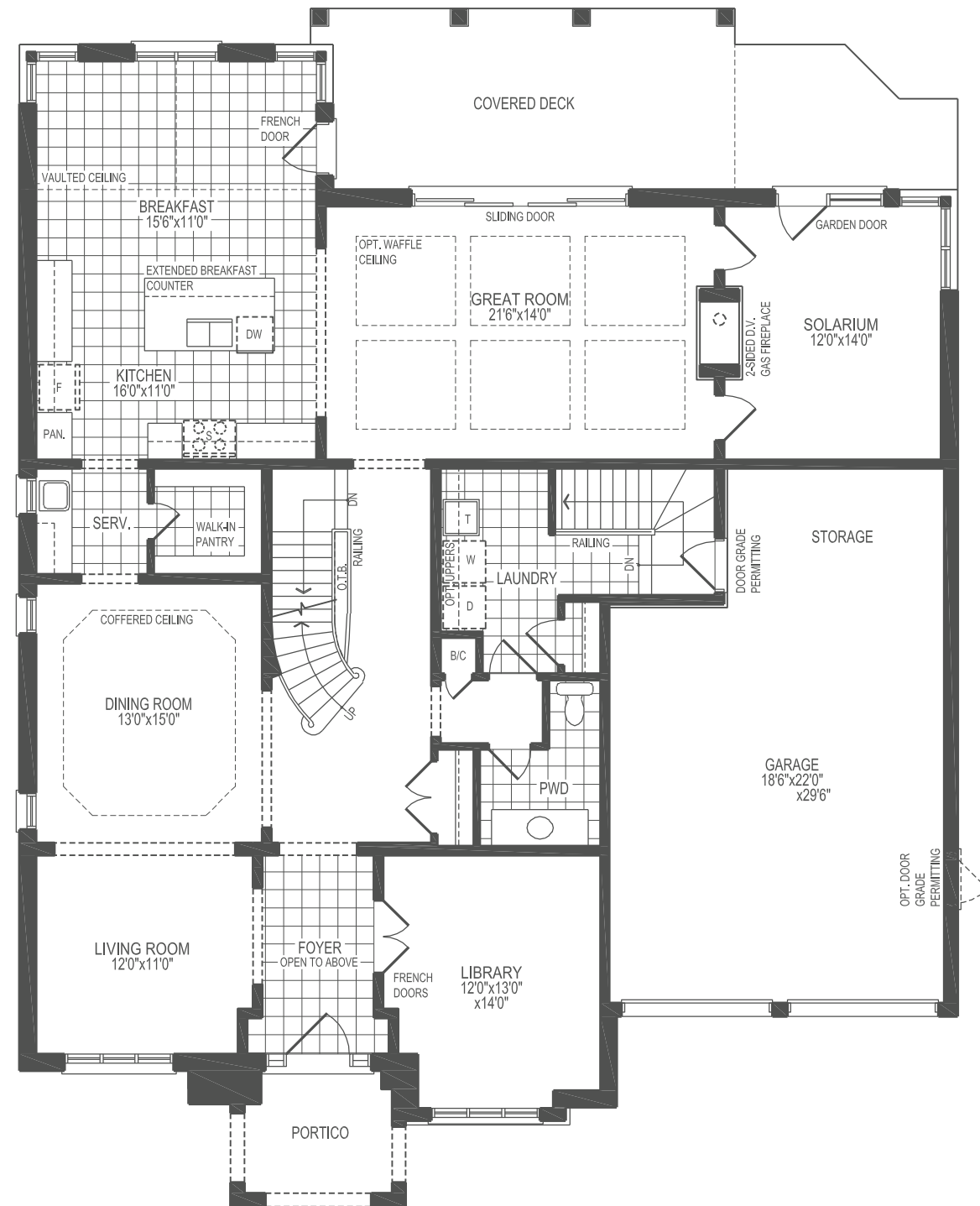
ALT. GROUND FLOOR PLAN EL. 'A' FOR LOTS 3 & 4 ONLY
