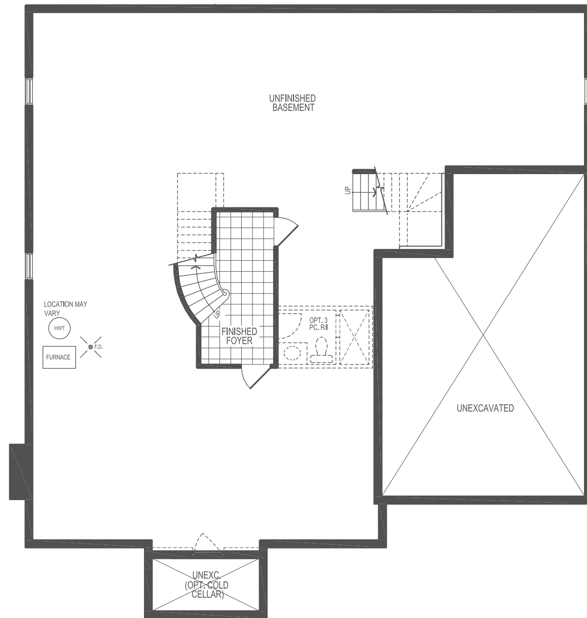
BASEMENT PLAN EL. 'B'
