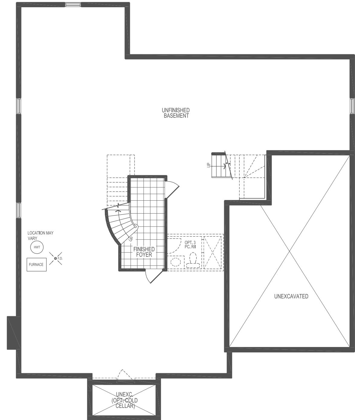
ALT. BASEMENT PLAN EL. 'B' FOR LOTS 3 & 4 ONLY
