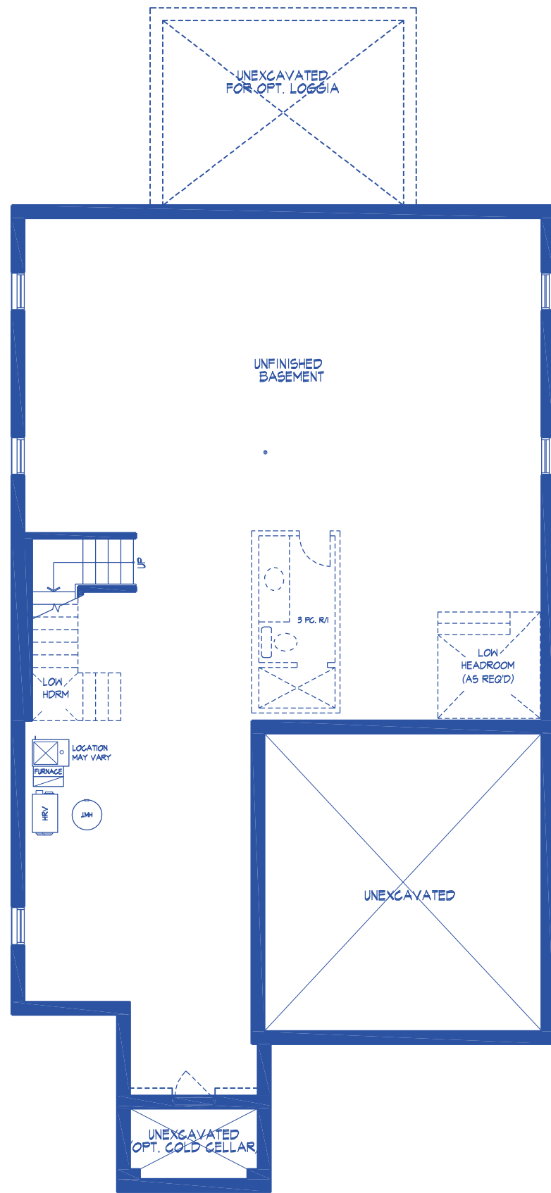
BASEMENT PLAN, EL. 'A' & 'B'
