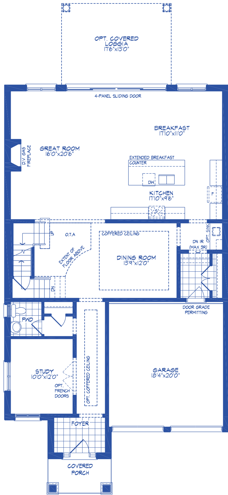
GROUND FLOOR PLAN, EL. 'A'
