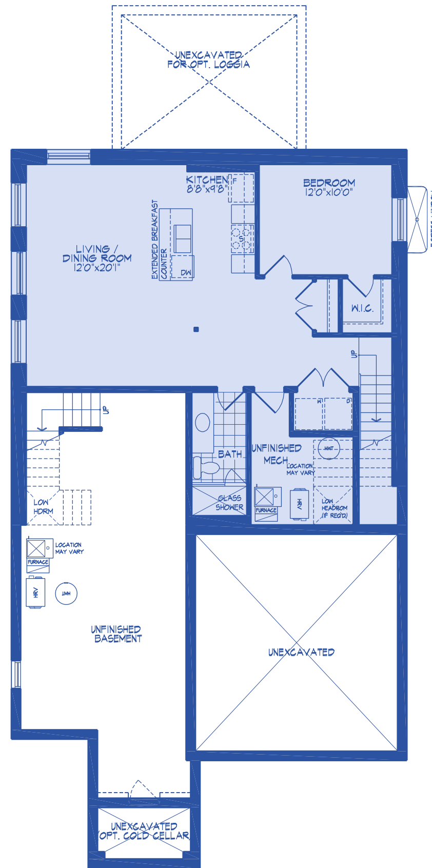
OPT. FLEX BASEMENT PLAN, EL. 'A' & 'B' (SIM. FOR EL. 'C')
