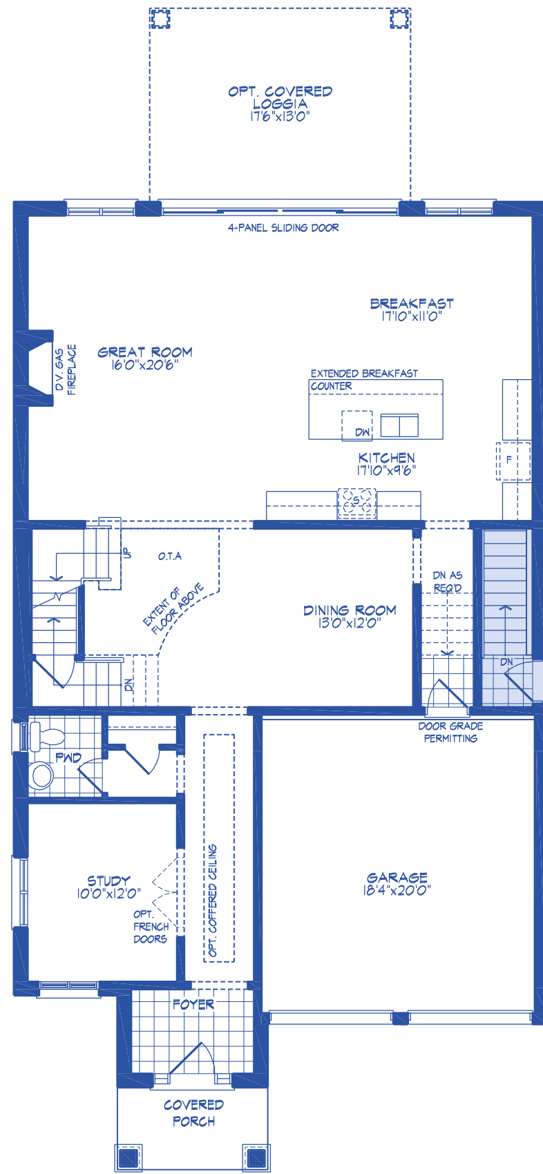
OPT. GROUND FLOOR PLAN, EL. 'A' (SIM. FOR 'B' & 'C') FOR OPT. FLEX BASEMENT
