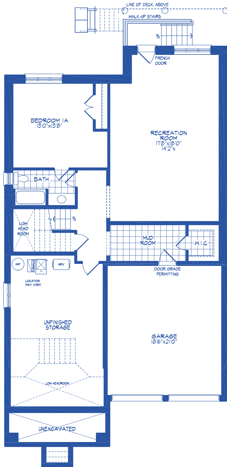
GROUND FLOOR PLAN, EL. 'C'
