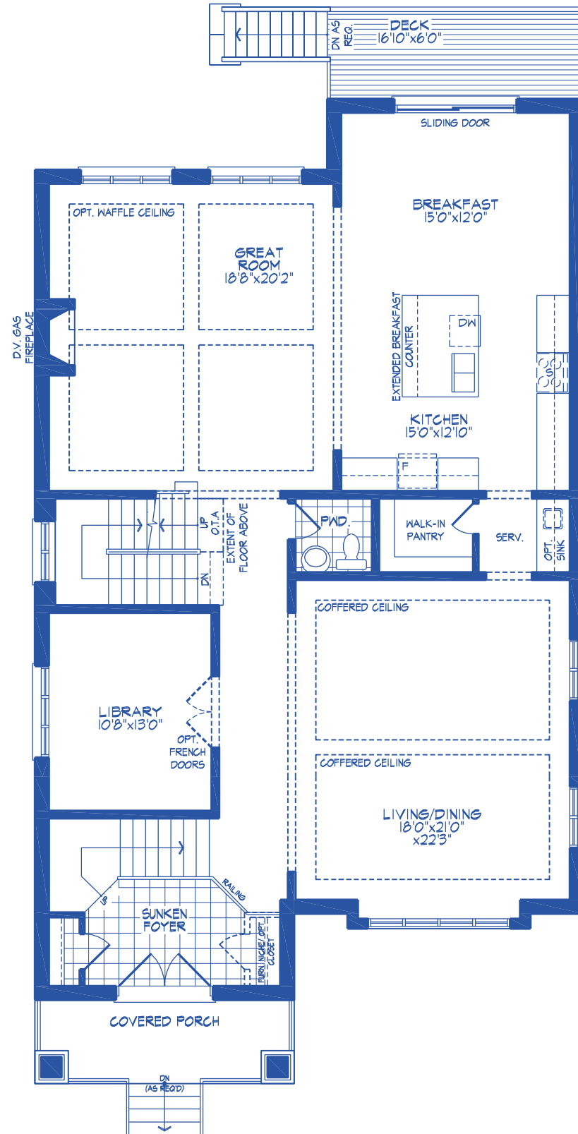
MAIN FLOOR PLAN, EL. 'C'
