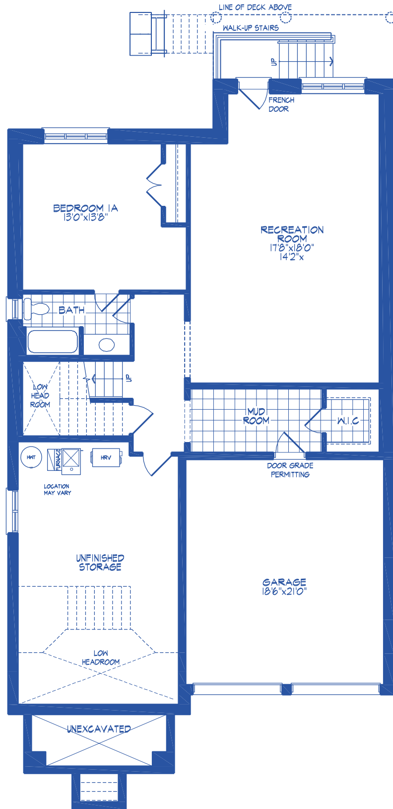
GROUND FLOOR PLAN, EL. 'B'
