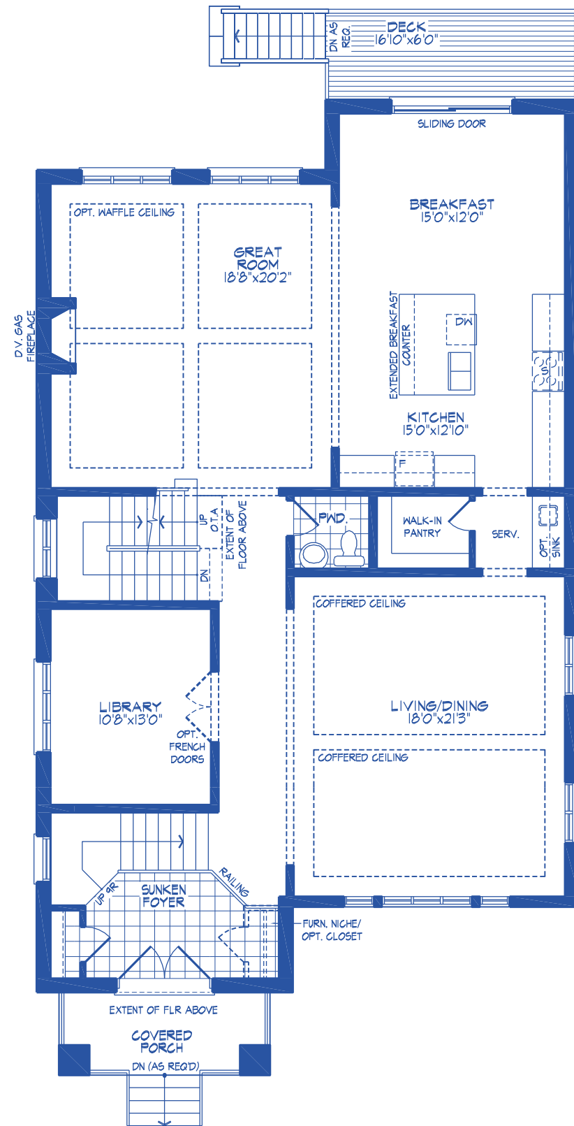
MAIN FLOOR PLAN, EL. 'B'
