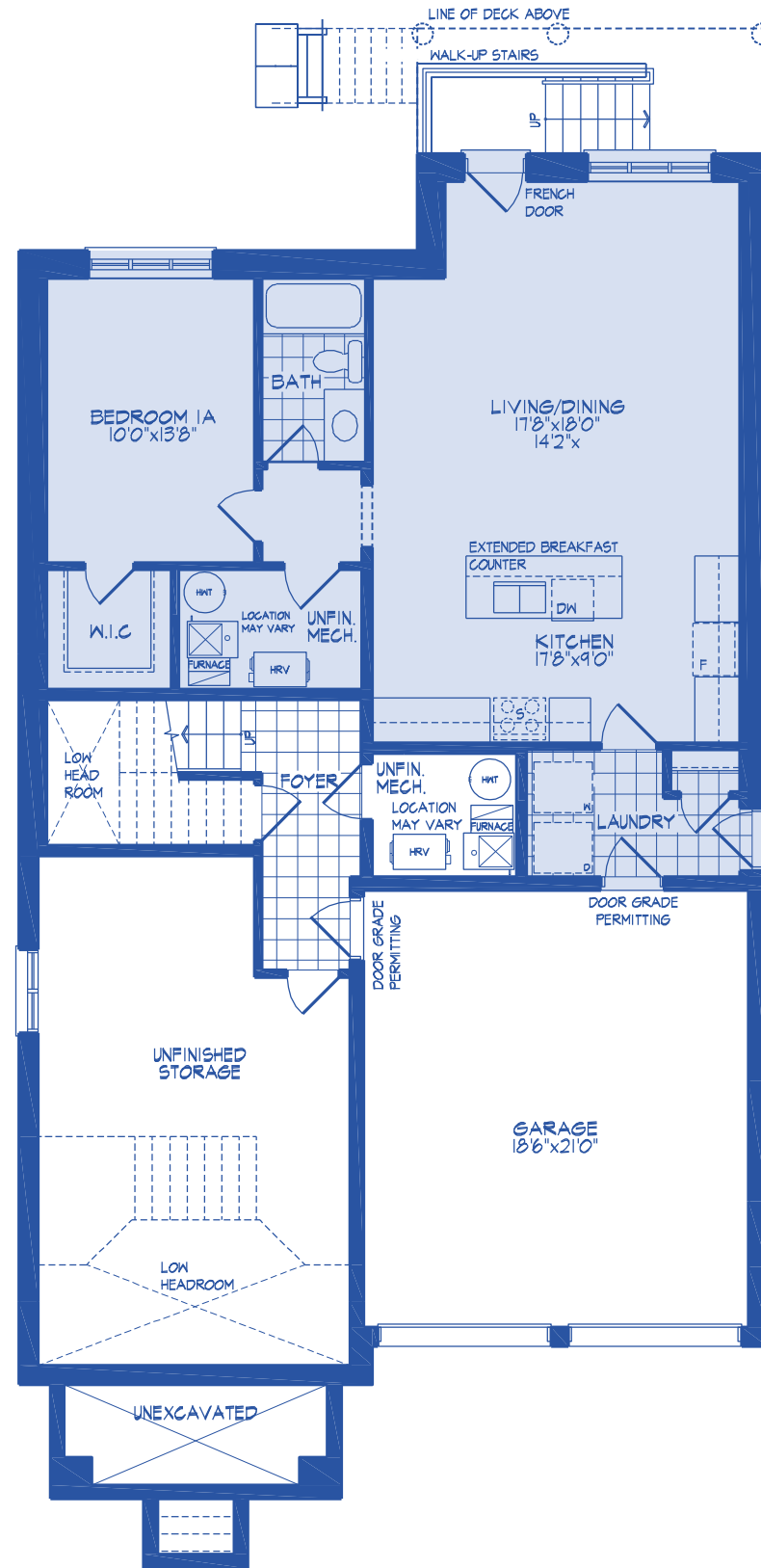
OPT. FLEX GROUND FLOOR PLAN, EL. 'B' (SIM. FOR EL. 'C')
