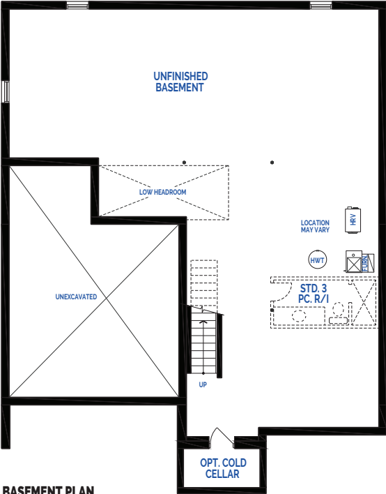
BASEMENT PLAN
